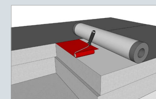
7 COSMO® SP-830.171 Bulbo bomba (Primer)
